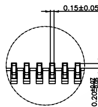
DETAIL C SCALE 3:1
